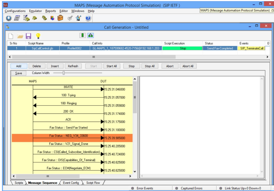
Figure: T.30 G.711 Pass through mode FAX simulation using MAPS™ SIP
