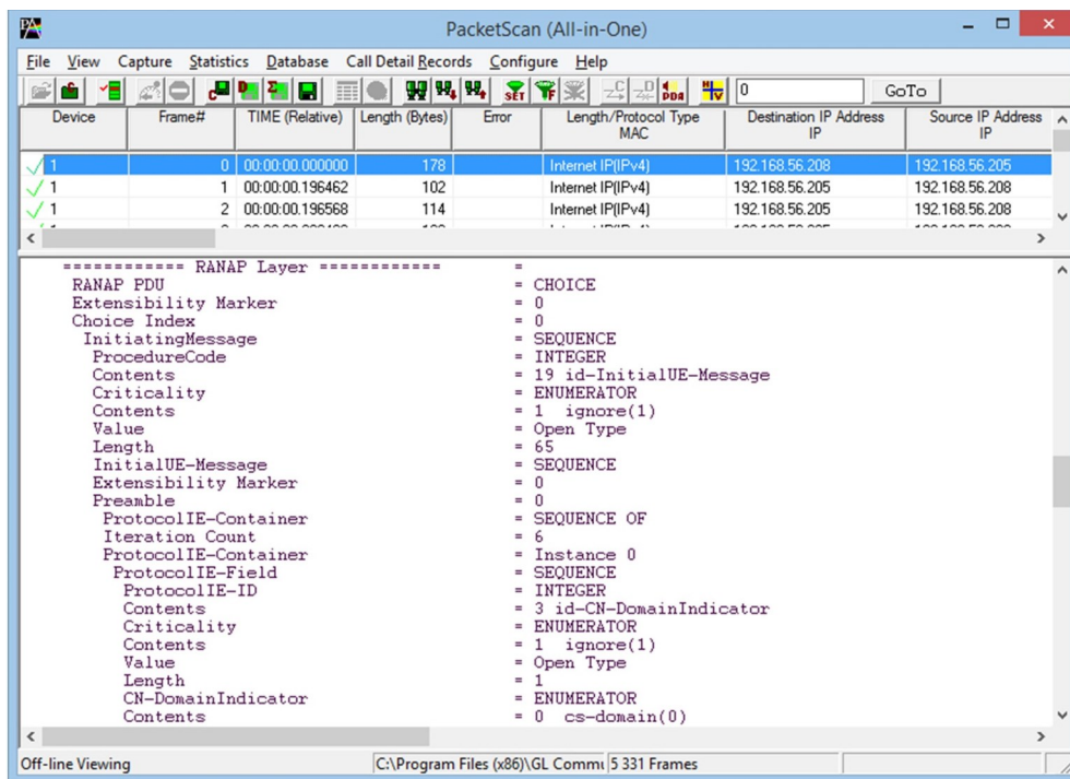
Figure: Detail View of UMTS luCS over IP
