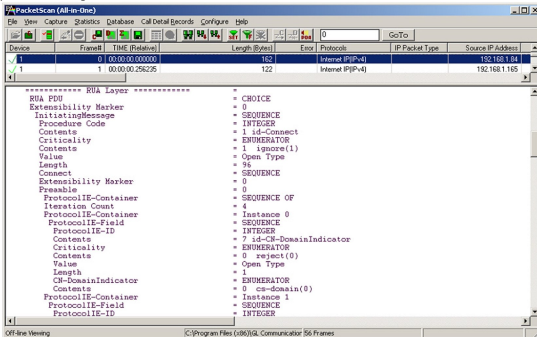
Figure: Detail View of UMTS luH over IP
