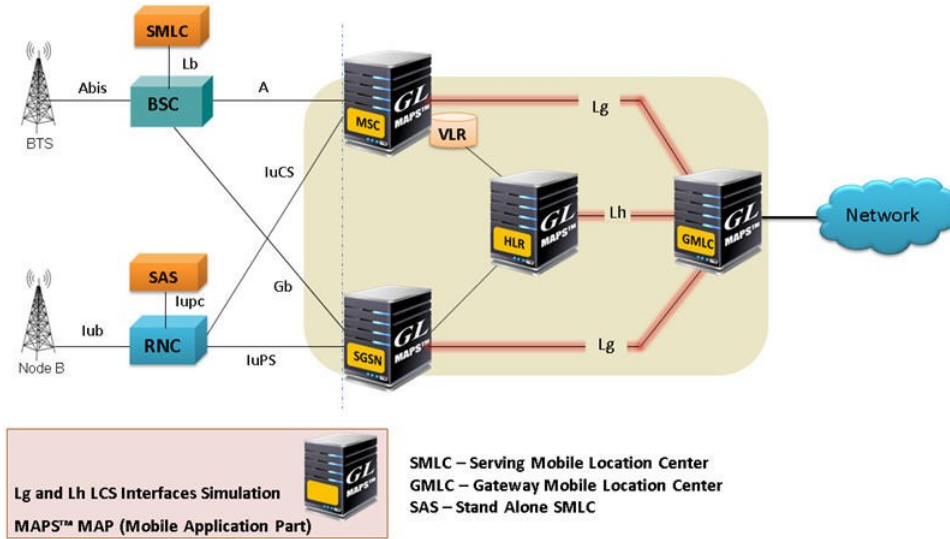
Figure: LCS Network Architecture
