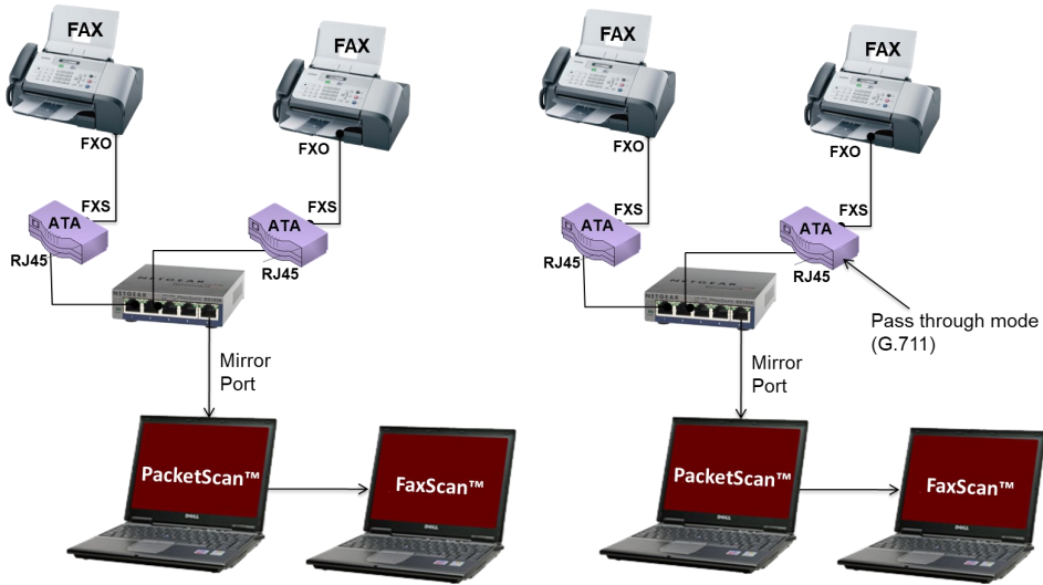
Figure: FAX Over IP T.38 and Pass-through Mode
