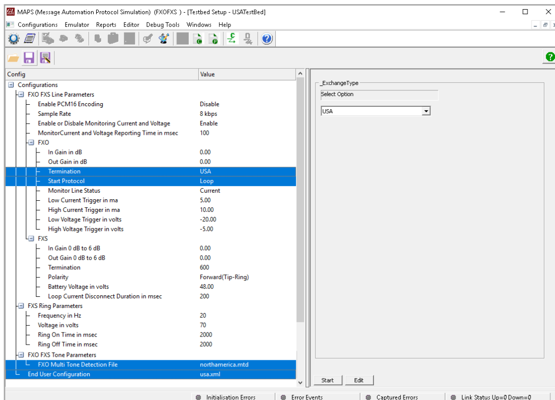
Figure: Tested Setup
