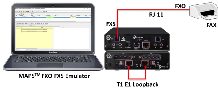
Figure: Send/Receive FAX over FXS Port
