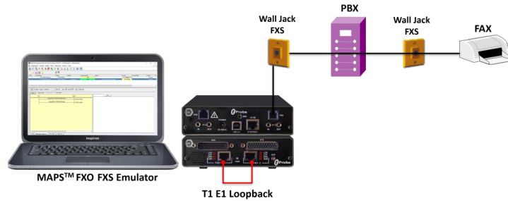
Figure: Send/Receive FAX over FXO Port
